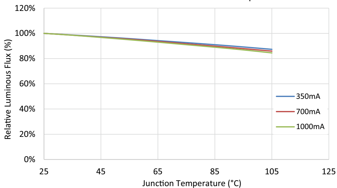
Relative Luminous Flux VS Junction Temperature
