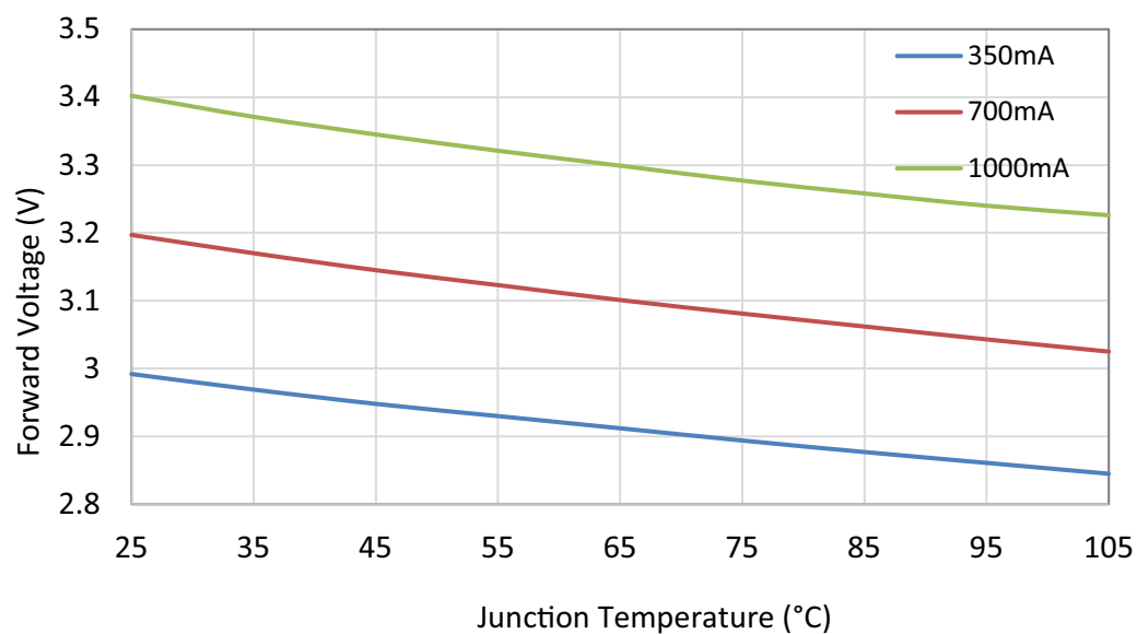
Forward Voltage VS Junction Temperature
