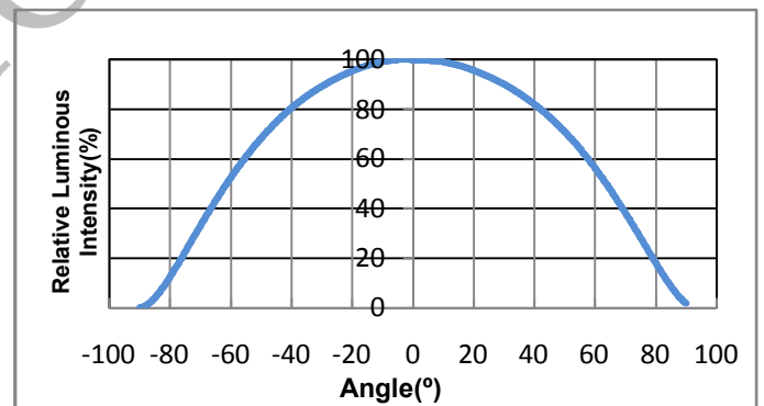
Fig.6- Radiation diagram
