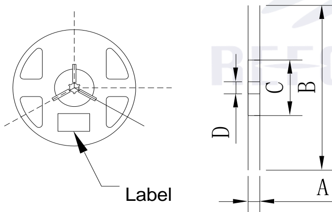
Fig.2-2 Reel Dimension
