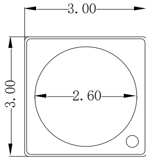
Fig.1-1 Top View
