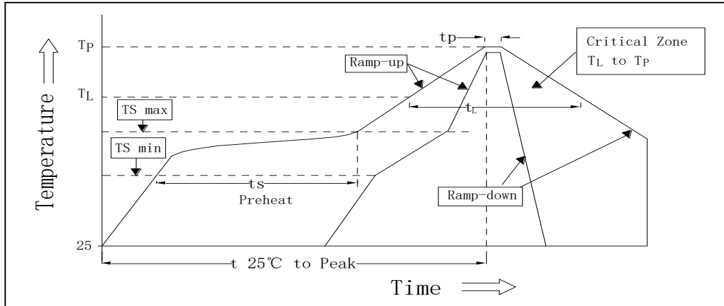
Fig.3-1 SMT Reflow Soldering Instructions
