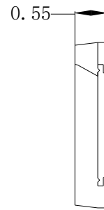
Fig.1-2 Side View
