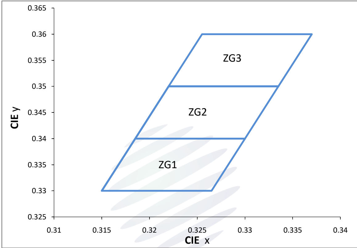
Fig. 1-6 The C.I.E Chromaticity Diagram
