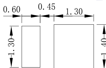
Fig.1-5 Soldering Patterns 推荐焊盘
