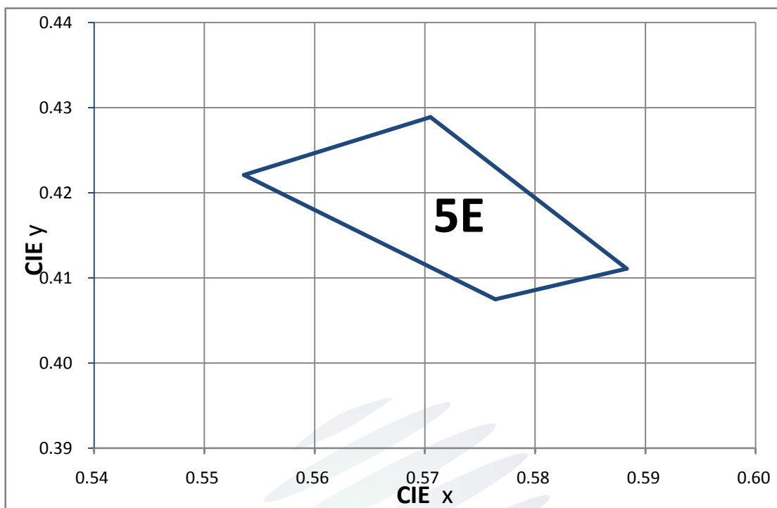
Fig. 1-6 The C.I.E Chromaticity Diagram
