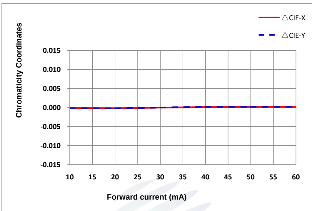
Fig. 1-13 Chromaticity Coordinate Shift Vs Forward Current
