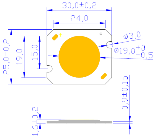
Outline dimensions
